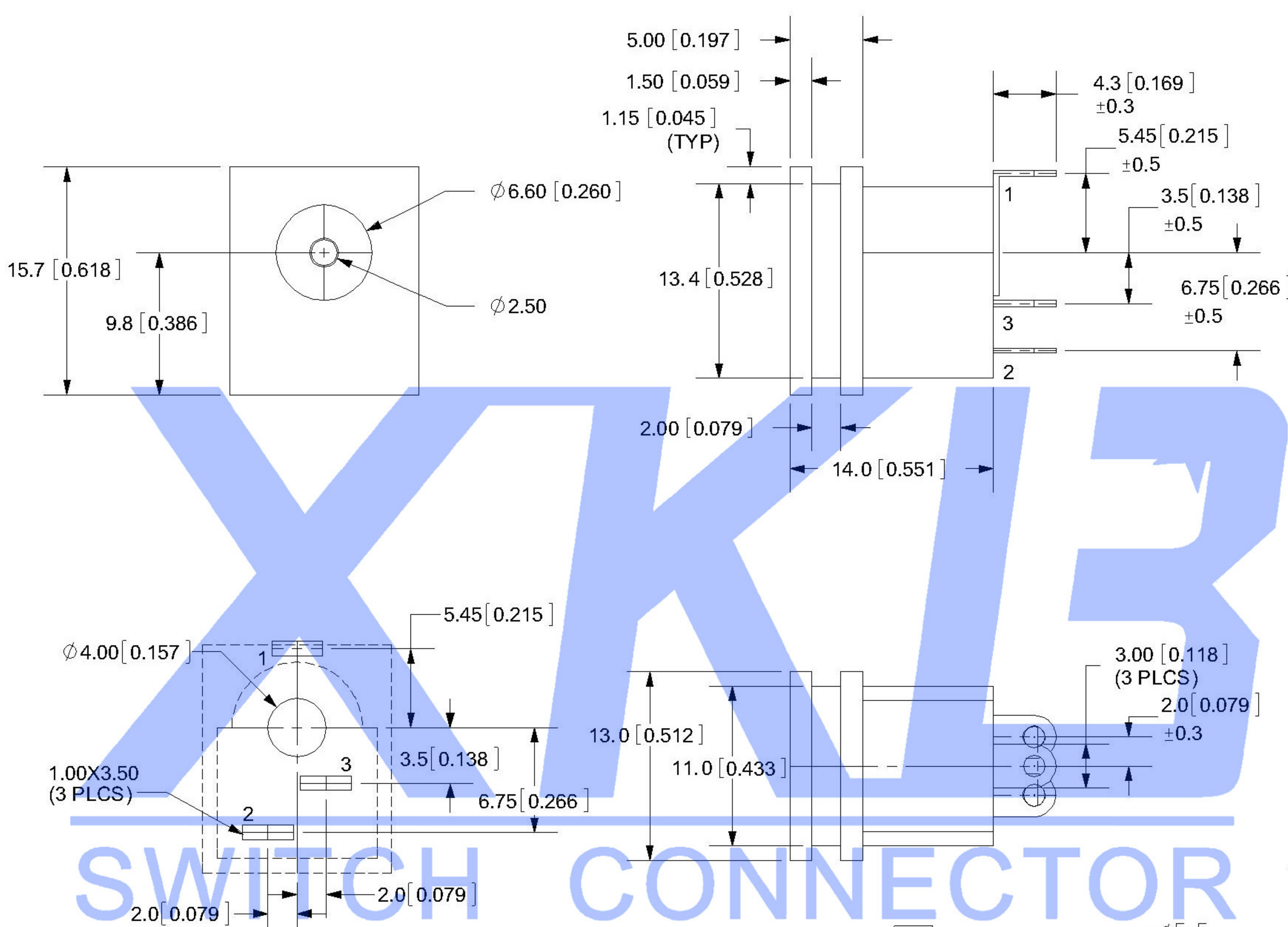
PCB LAYOUT FRONT VIEW
